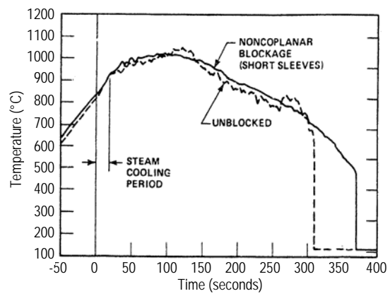
Figure 12: FLECHT-SEASET 21 rods. Steam temperature for unblocked and non coplanar blockage (short sleeves) configurations.
