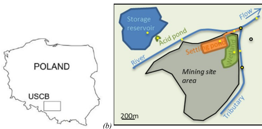
FIG. 1: Localization of the Upper Silesian Coal Basin (USCB) in Poland (a) and scheme of the coal mining area including the pond identified as "storage reservoir" (b); sampling points were illustrated by yellow dots.
